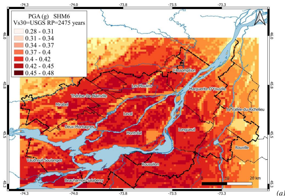
Figure 2. PGA (in g) calculated on a regular grid using SHM6 for the return period of 2475 years (probability of exceedance of 2% in 50 years) integrating the V_{s30} data in Figure 1 from the USGS.
