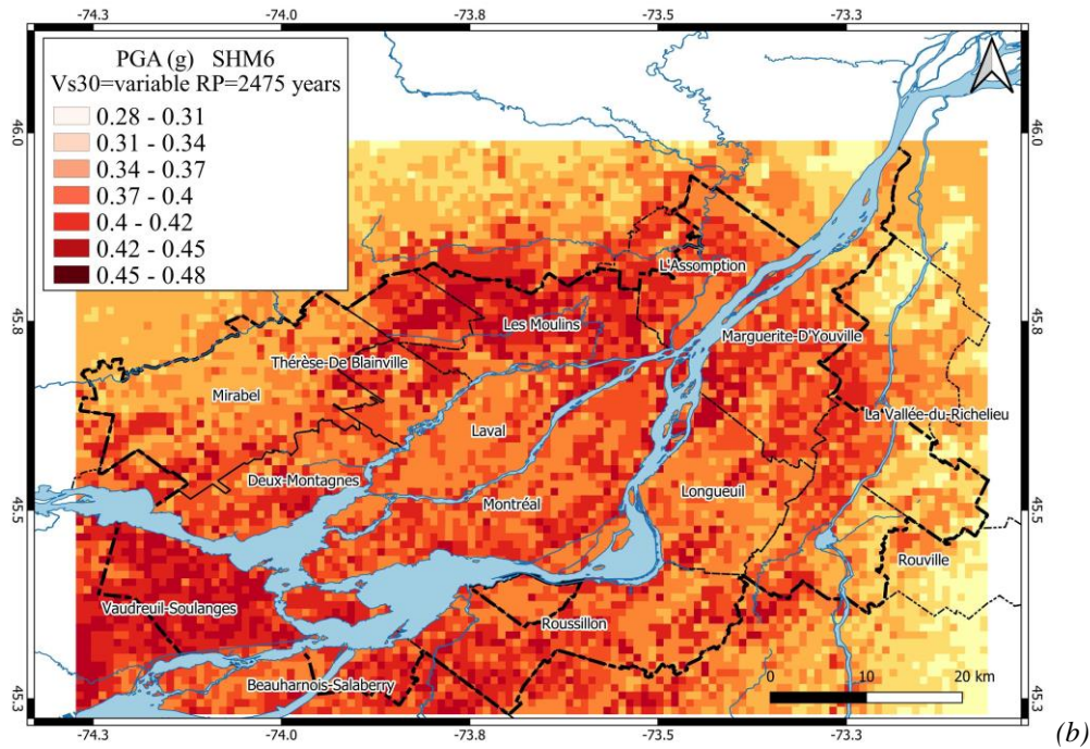
Figure 2 (continue). PGA (in g) calculated on a regular grid using SHM6 for the return period of 2475 years (probability of exceedance of 2% in 50 years) integrating the V_{s30} data in Figure 1 from the detailed maps.
