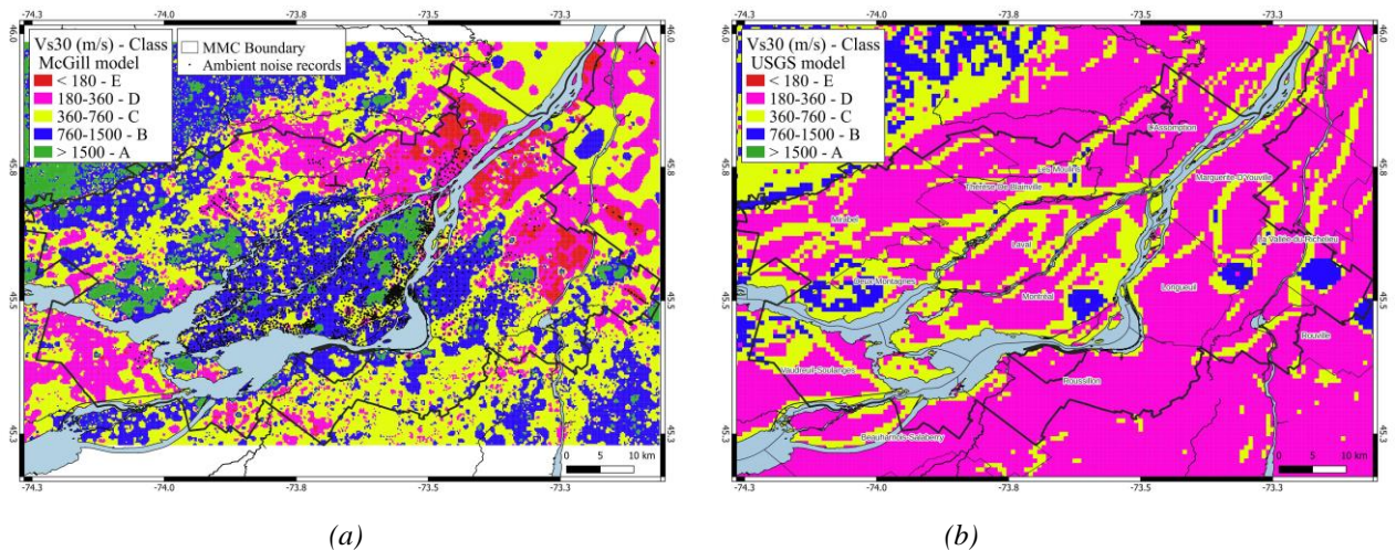
Figure 1. Site models in Greater Montreal in terms of V_{s30} (in m/s) grouped in site classes from (a) the detailed map and (b) the USGS data.
