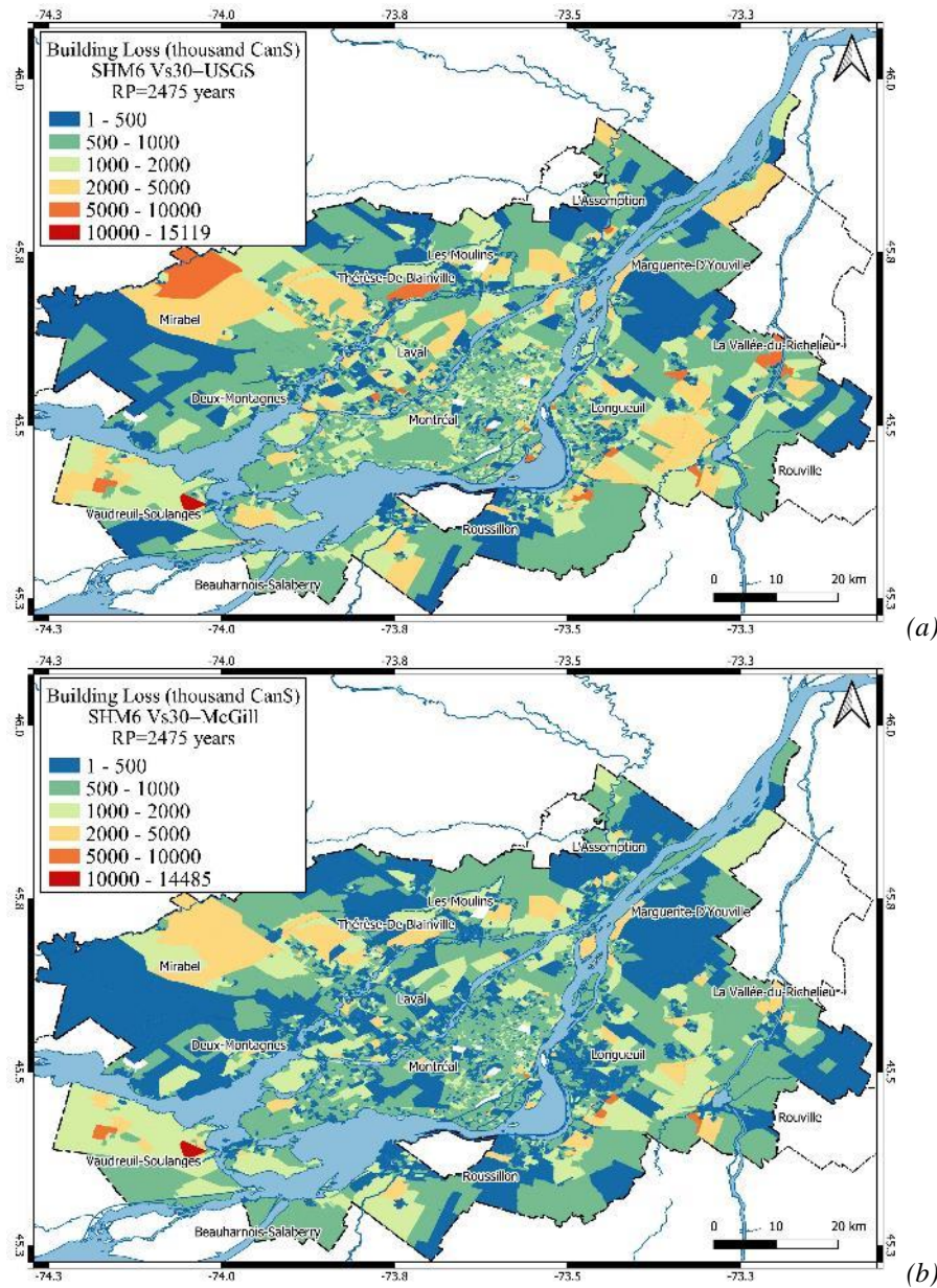
Figure 4. Residential building loss by DA calculated using SHM6 for a probability of exceedance of 2% in 50 years integrating the V_{s30} data in Figure 1 from (a) the USGS and (b) the detailed maps.
