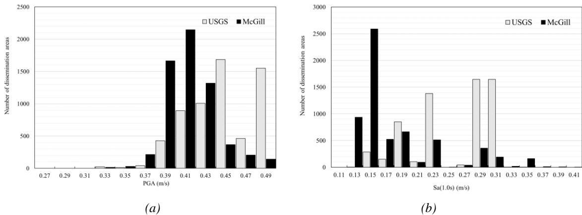
Figure 3. Distribution of calculated (a) PGA and (b) S_a(1.0s) by DAs using SHM6 for the return period of 2475 years (probability of exceedance of 2% in 50 years) and the V_{s30} models from USGS and McGill.
