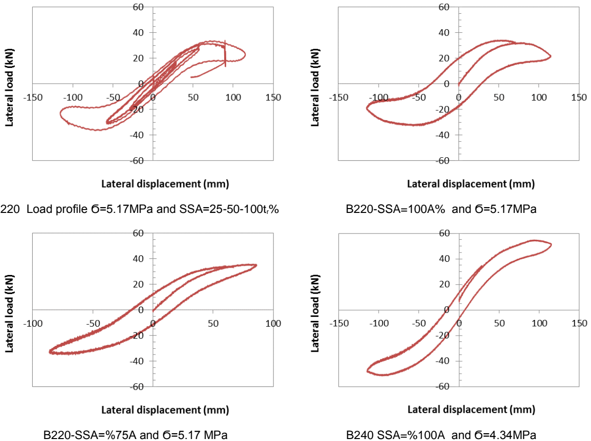
Fig. 6 - Force-Displacement Hysteresis Diagram of B220 and B240 isolators under constant pre-load of 250 KN (SSA=50-75-100%,t,)
