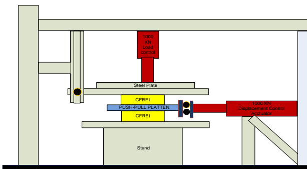
(a) schematic of dual shear test configuration
