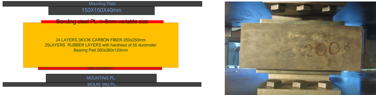
Fig. 1 - ESB-CFREI with top and bottom experimental mounting Plates (left) and ESB-CFREI isolator (right)
