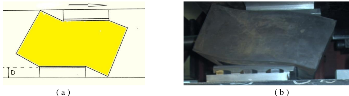
Fig. 2 – Schematic (left) and experimental (right) deformation mechanism of ESB-CFREI under lateral shear load ( D = distance Isolator's bearing pad is elevation from the supports)
