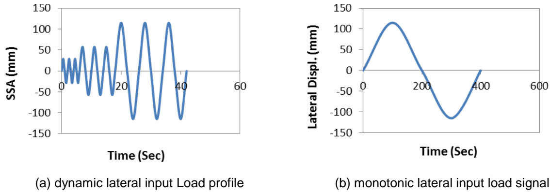
Fig. 5 - Lateral cyclic input load signals- (SSA = 25%, 50% & 100%t, or 28.75, 57.5 & 115mm) under constant axial compression pre-load of Pv = 250kN)
