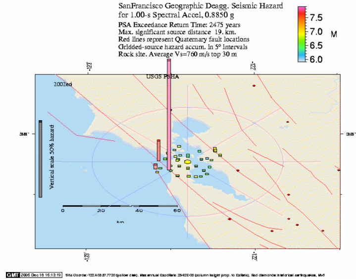
Figure 3. Deaggregation for San Francisco, California.
