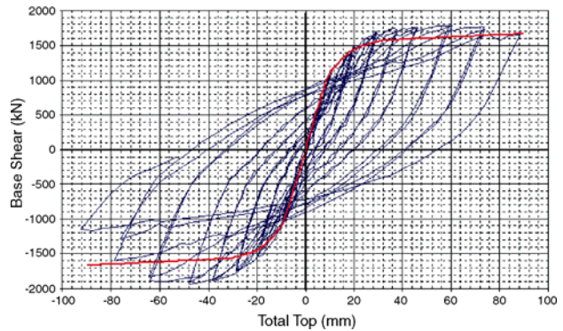
Figure 5. SPSW Specimen with Cutout Corners (right) and Typical Hysteresis Loops for Solid Wall Specimen (Vian and Bruneau 2004).
