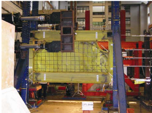
Figure 5. SPSW Specimen with Cutout Corners (right) and Typical Hysteresis Loops for Solid Wall Specimen (Vian and Bruneau 2004).
