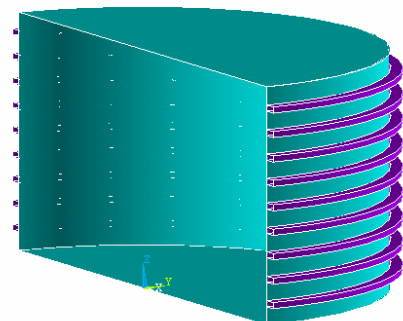
b) Elastomeric isolators with outer steel rings
