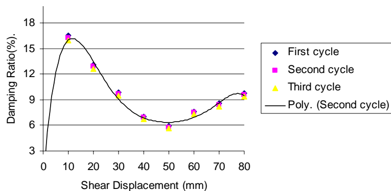
Figure 9. Shear effective damping ratio-displacement relation.
