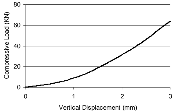
b) Vertical load-displacement relation actuator
