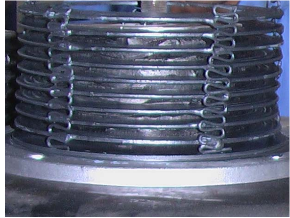
b) Rubber penetrates among the rings with assembling meandering bars
