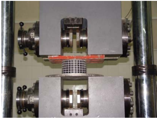
a) Test set up 1
