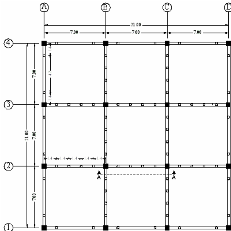
Figure 1. Isolators locations on beams for each story in case 1.
