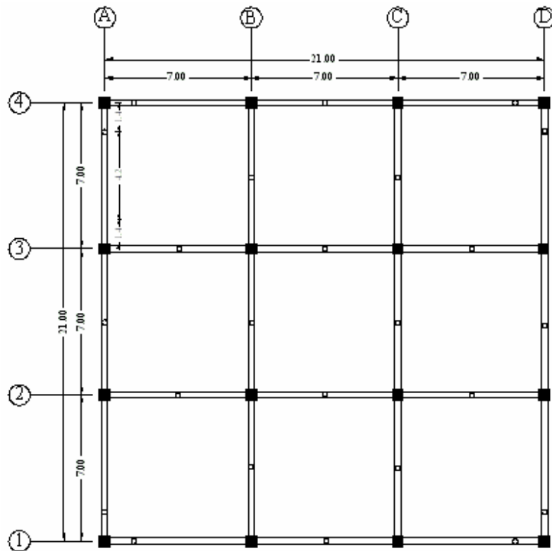
Figure 2. Isolators locations on beams for each story in case 2.
