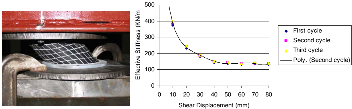
a) Deformation shape in displacement 80mm b) Shear Effective Stiffness-displacement relation
