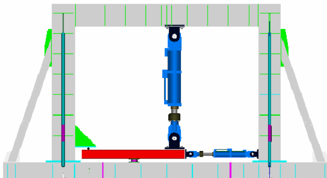
a) Schematic model
