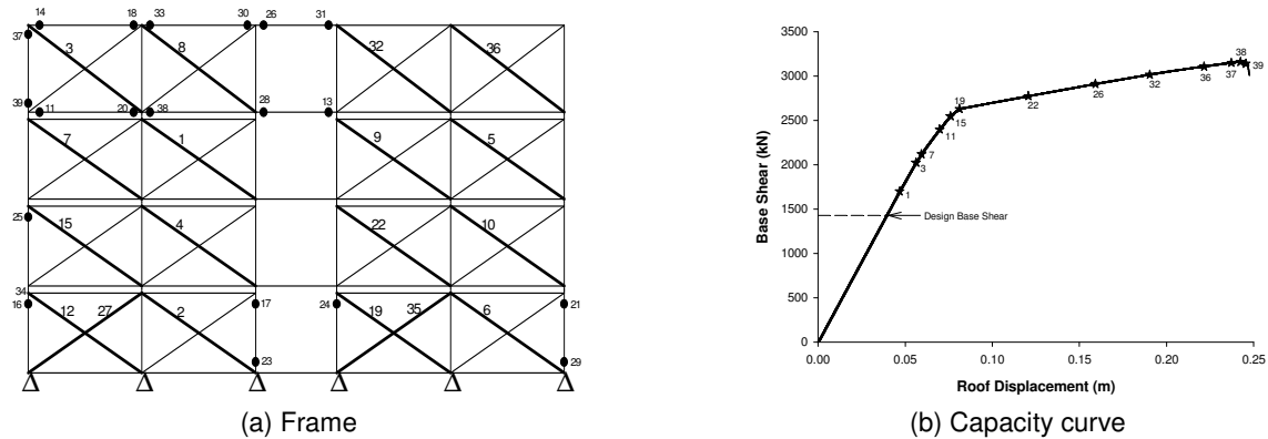
Figure 3. Sequence of yielding/buckling of the 4-storey MSB braced frame (brace induced column actions by SRSS accumulation approach).
