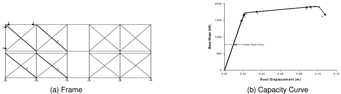
Figure 4. Sequence of yielding/buckling of the 2-storey MSB braced frame (brace induced column actions by SRSS accumulation approach).
