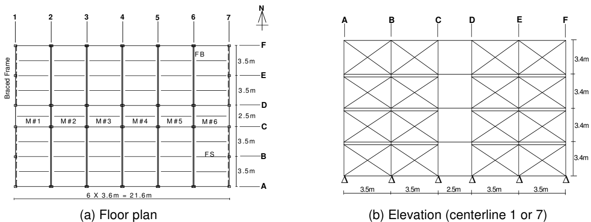
Figure 2. 4-storey modular steel braced frame.
