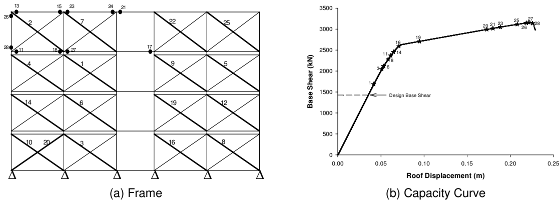
Figure 5. Sequence of yielding/buckling of the 4-storey MSB braced frame (brace induced column actions by DS accumulation approach).
