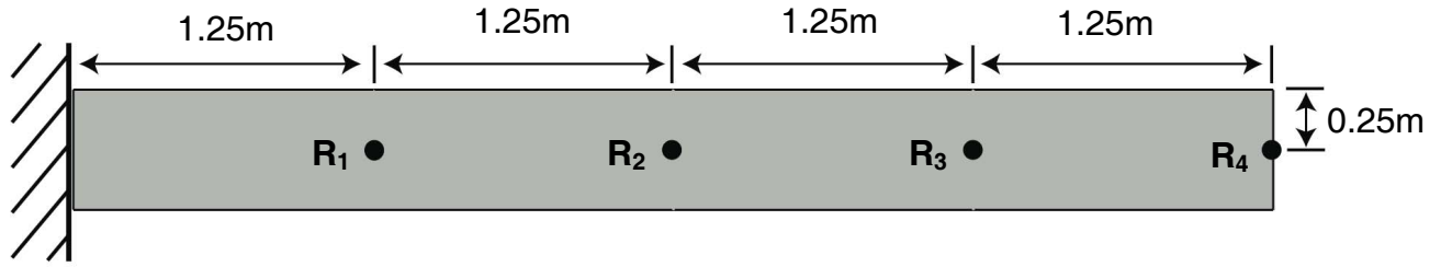
Figure 2. Receiver locations. Receivers are equally spaced along the beam's center axis.
