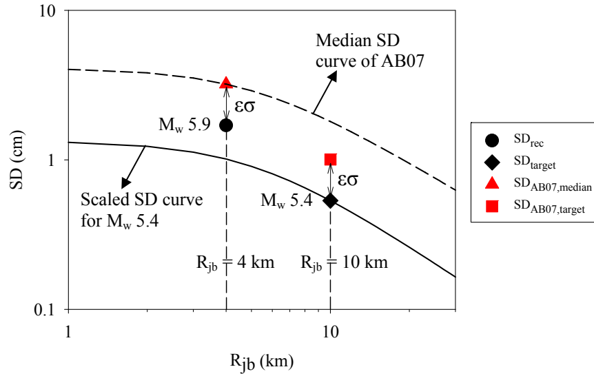
Figure 1. A scaling example to describe Method 1.
