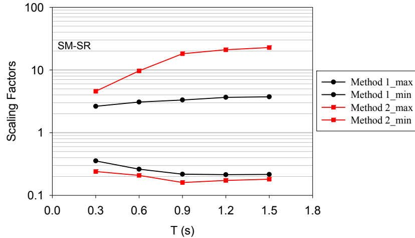
Figure 5. Maximum and minimum scaling factors computed by Methods 1 and Method 2.
