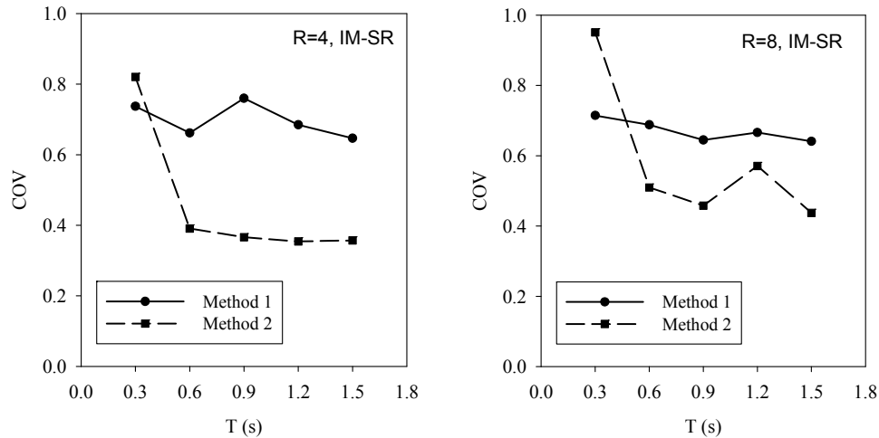
Figure 4. COV statistics of SDOF systems as a function of vibration period with different level of inelasticity.
