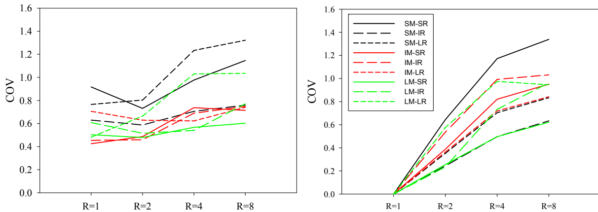
Figure 3. COV statistics computed at T = 0.6s for constant strength values varying between R = 1 (elastic behavior) to R = 8 (highly nonlinear behavior).
