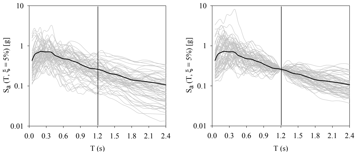
Figure 2. Scaling to the bin-median spectral acceleration according to Method 2. Black line presents the average acceleration spectrum of IM-SR bin.
