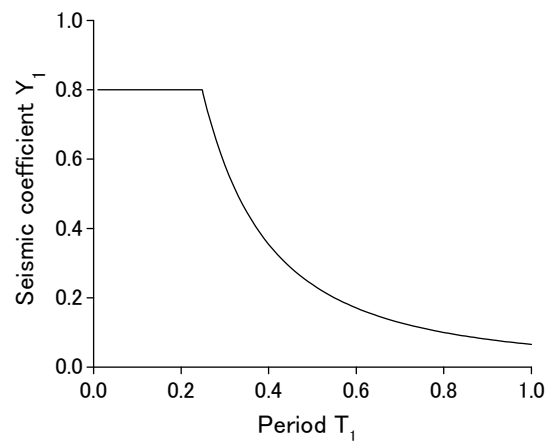
Figure 1. Relationship between the initial elastic period, T_1 and the seismic coefficient, Y_1 .
